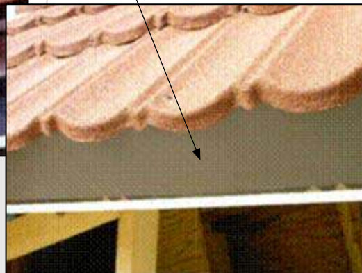
Wide-faced (5-in.) stone-coated or painted metal fascia covers batten framing on roof over applications. The flashing is narrower (3-in. deep) on new construction.
