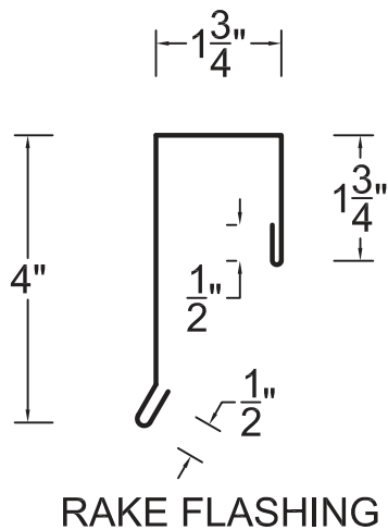
DRAWING: CB 11 RAKE
