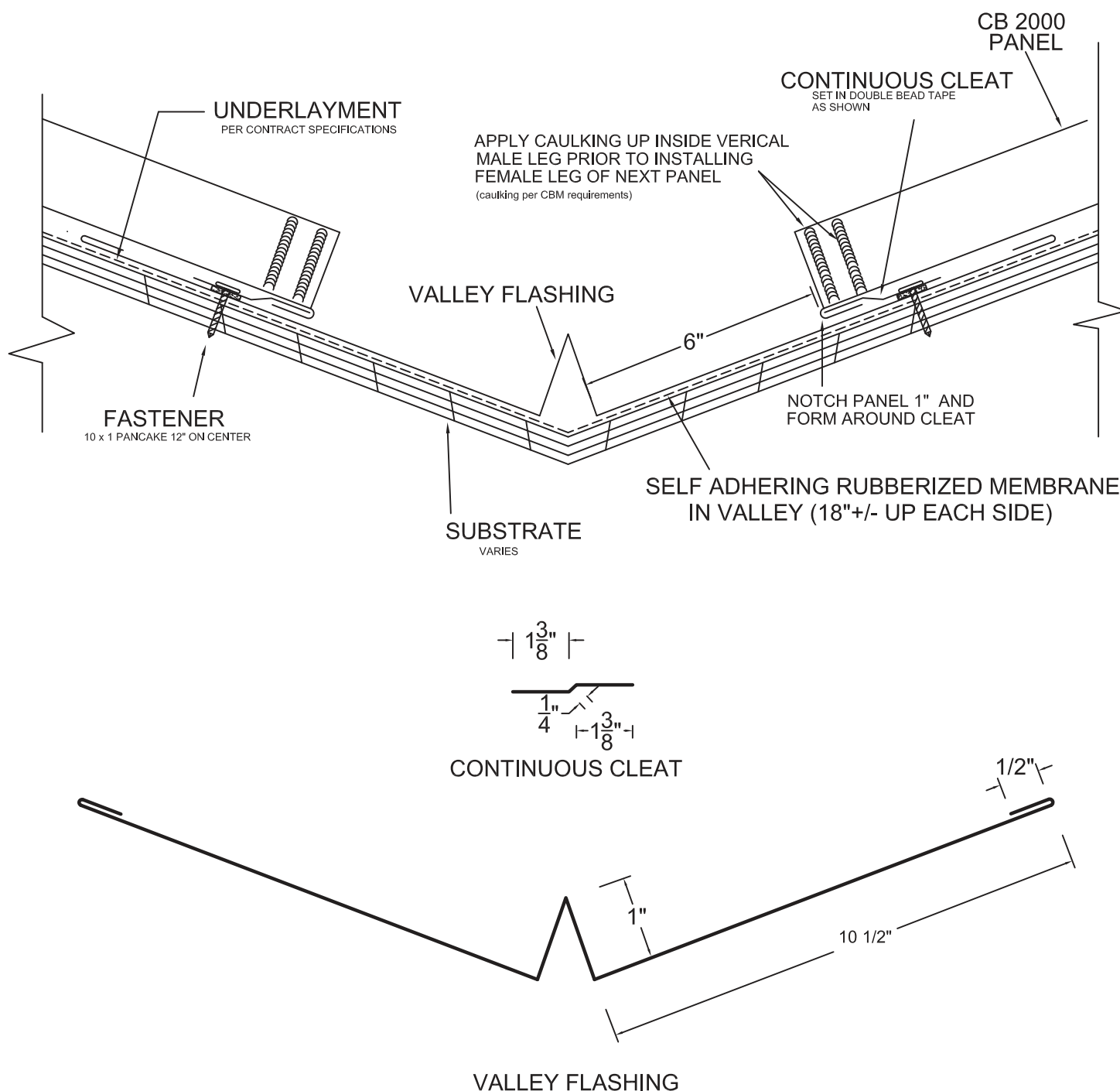
DRAWING: CB 10 VALLEY cleat
