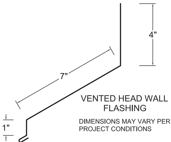
DRAWING: CB 15 HEADWALL- VENTED
