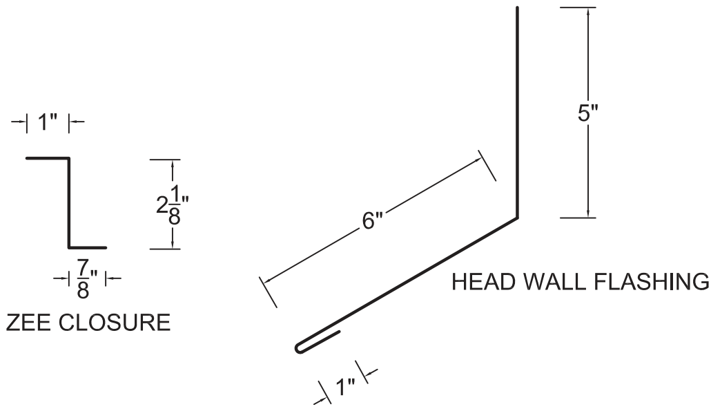
DRAWING: CB 14 HEADWALL
